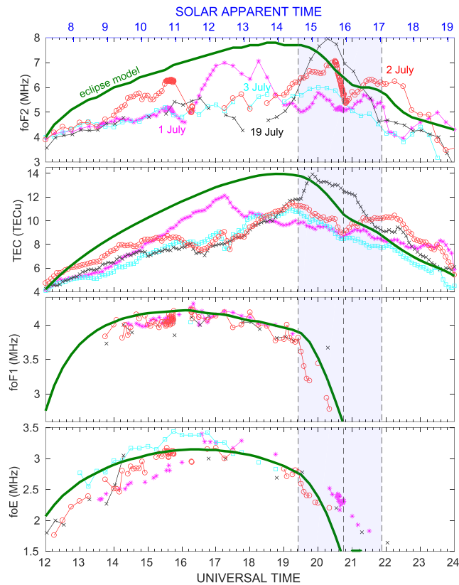
Figure 8. SUPIM-INPE simulations of foF_2 , foF_1 , foE , and TEC without the prereversal electric field during the 2 July 2019 eclipse (solid green line) at La Serena (29.9°S, 71.3°W) and observations on 1 (stars), 2 (open circles), 3 (open squares), and 19 July 2019 (crosses).
