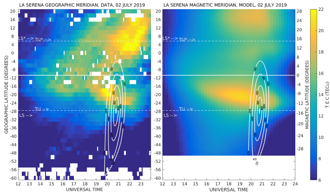
Figure 6. Latitude-time TEC distribution along the La Serena (LS: 29.9°S, 71.3°W) geographic meridian (observations, left) and geomagnetic meridian (SUPIM-INPE model, right). The eclipse path and its interval are highlighted with white contours, representing the latitudinal sections and the corresponding times with 20%, 40%, 60%, 80%, and 100% eclipse obscuration at 300 km altitude. Magnetic equator (horizontal continuous line). Geomagnetic latitudes \pm 15^\circ (horizontal dashed lines). La Serena (LS), Tucumán (TU: 26.9°S, 65.2°W), and corresponding geomagnetic conjugate latitudes (arrows).
